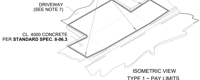
"CEMENT CONCRETE DRIVEWAY ENTRANCE TYPE 1" PAY LIMITS
