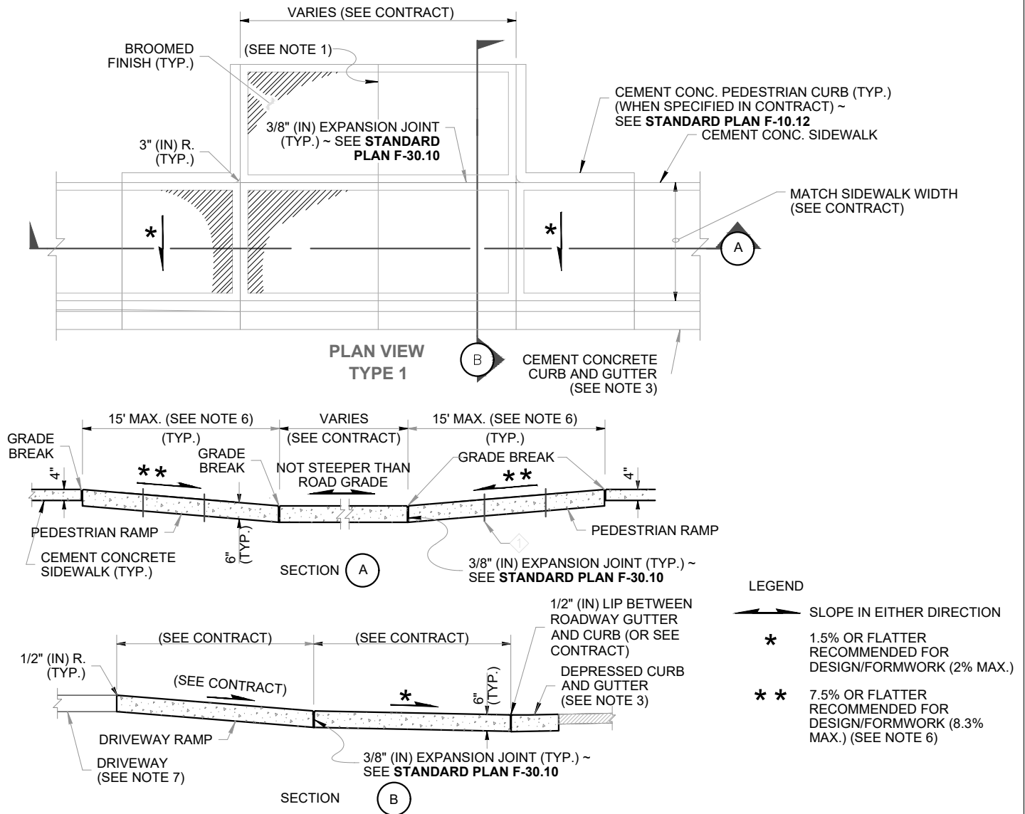
"CEMENT CONCRETE DRIVEWAY ENTRANCE TYPE 1" PAY LIMITS
